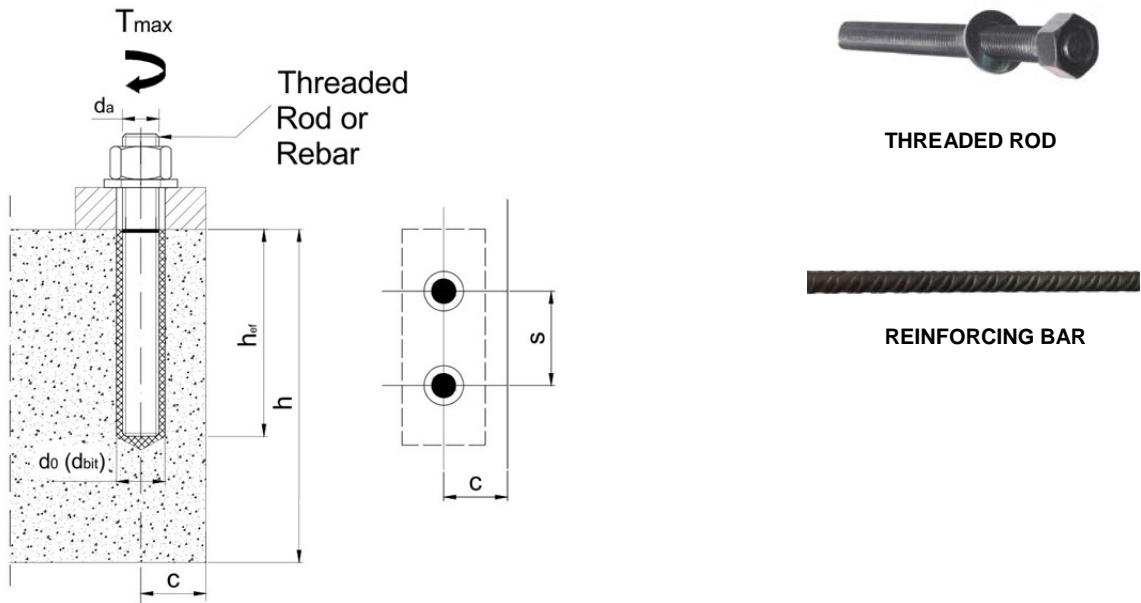
FIGURE 1—INSTALLATION PARAMETERS FOR THREADED RODS AND REINFORCING BARS
